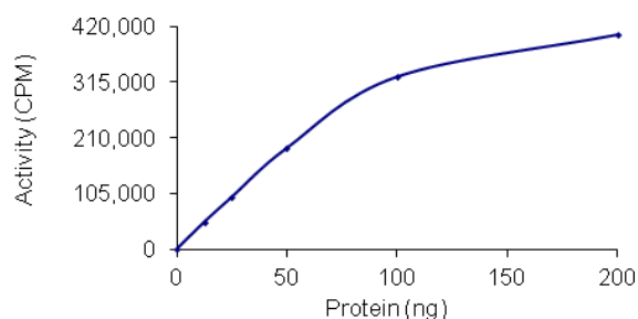
Figure 2. Specific Activity of Lot Number SLBB2532: 190 nmole/min/mg
